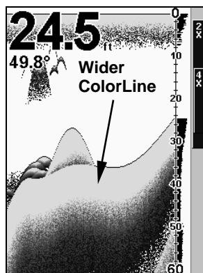
Little ColorLine (left) indicates a soft bottom, probably sand or mud. The wider ColorLine (right) indicates a harder, rocky bottom.
